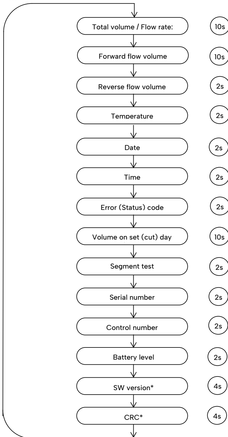
Figure 6.1 Menu structure in User mode
